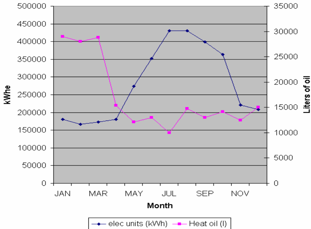
Chart 2. Energy Load profile of a typical Hotel
